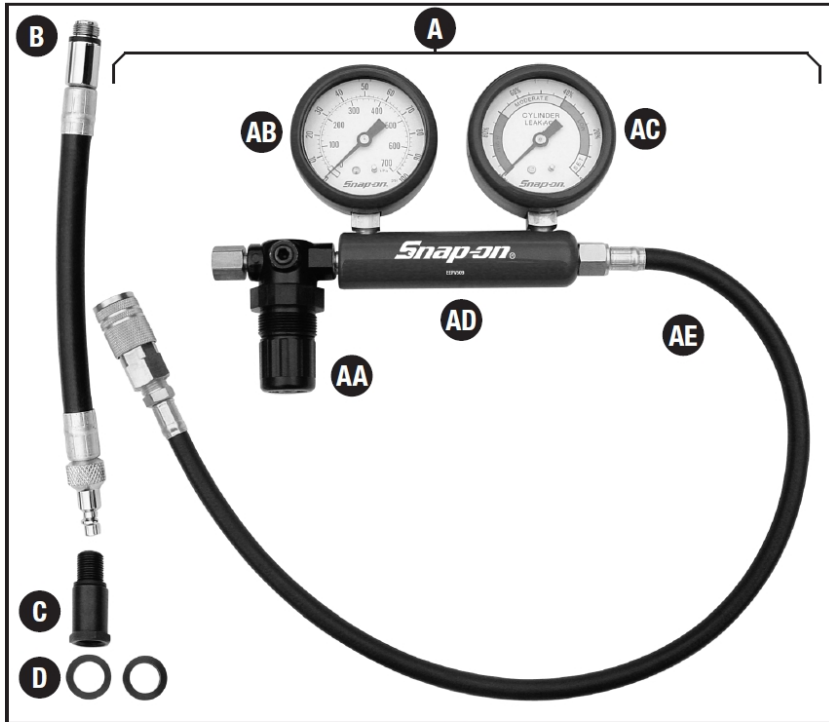
Figure 1: EEPV509 Cylinder Leakage Tester
